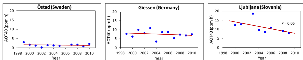
Figure 37: Trend in AOT40 at three selected sites in Europe. A significant trend ( P = 0.06 ), a decline of 0.6 ppm h per year, was found only in Ljubljana (Slovenia).
