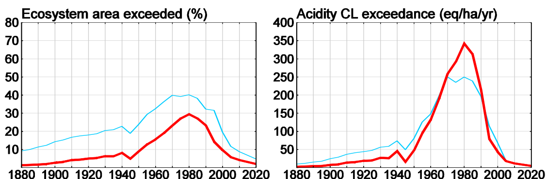
Figure 26: Temporal development of the area in Europe where acidity critical loads are exceeded (left; % of ecosystem area) and average accumulated exceedance (AAE) (right; \text{eq ha}^{-1} \text{yr}^{-1} ) of critical loads of acidity (red: all ecosystems, blue: surface waters). Future exceedances are based on the implementation of agreed legislation (emission and deposition data from EMEP-CIAM and EMEP- MSC-W; critical loads data from the CCE).
