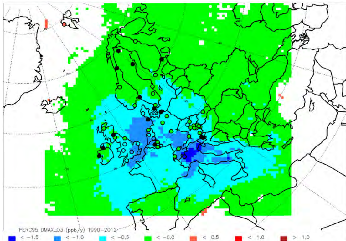
Figure 34: Sen's slopes ( \text{ppb year}^{-1} ) of the modelled annual 95 percentiles of the daily maximum ozone concentration for the period 1990–2012 with the results from EMEP monitoring data on top (circles). The colors indicate the magnitude of the trend. Filled, black circles indicate non-significant slopes. Note that the significance criteria for the stations were changed from p=0.05 to p=0.2 in this plot.
